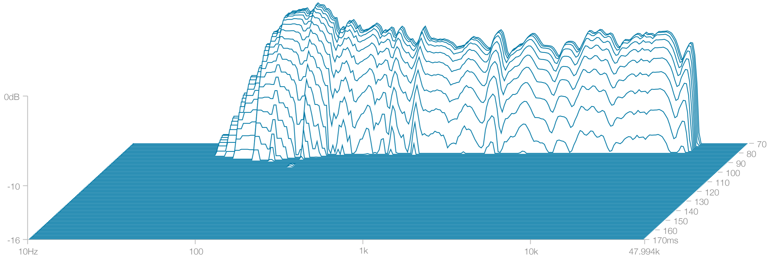
FFT Waterfall (1/24 Octave Smoothing)
