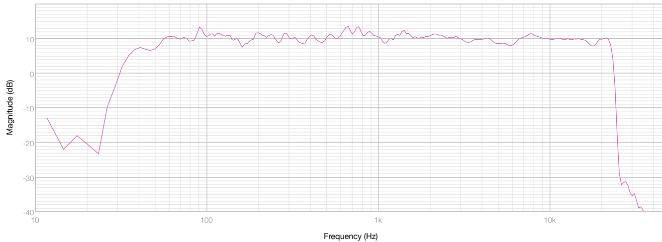
Frequency Response (1/24 Octave Smoothing)
