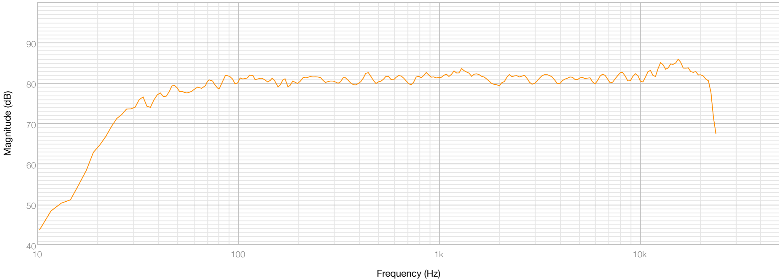
Sound Pressure Level (1/24 Octave Smoothing)
